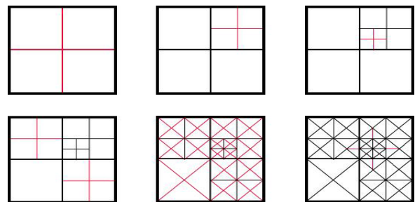
Figure 2: Branching Restricted Quad-Tree, from left to right: a-) 1.LOD, b-) 2.LOD, c-) 3.LOD, d-) Level Refinement, e-) Triangulization, f-) Connecting levels
